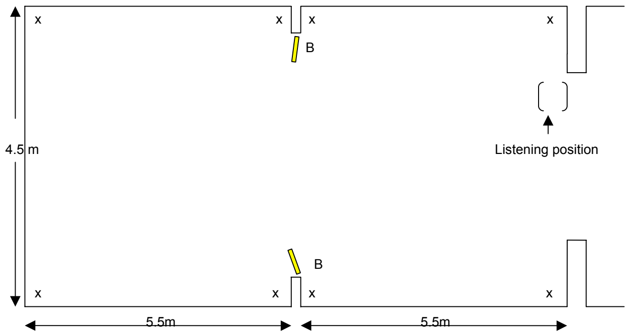
FIG 1.1: listening room floor plan.
